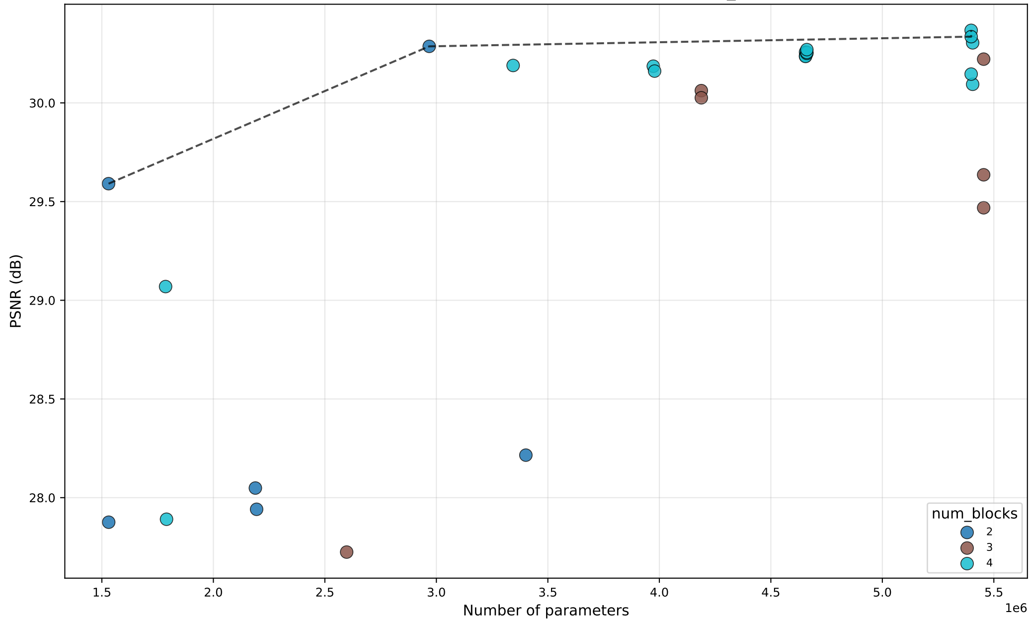
PSNR vs #Params — WaveletAttention — by num_blocks
